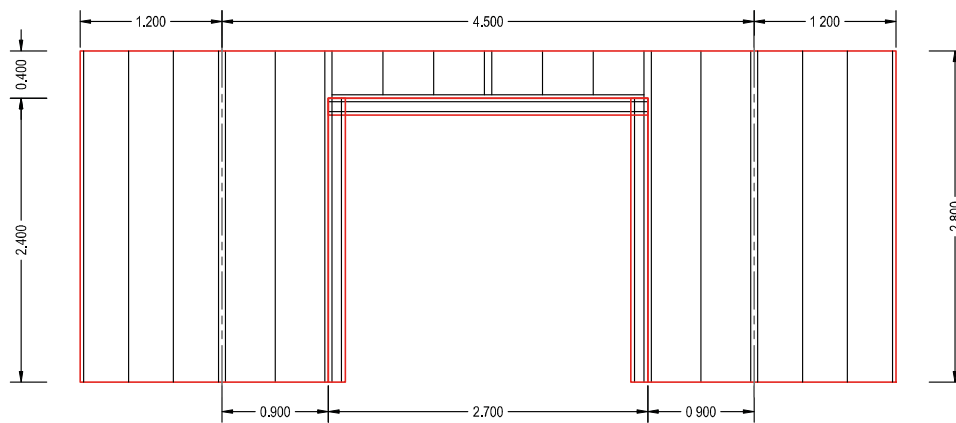
LAYOUT JOISTS
