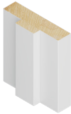
STANDARD DOOR FRAME PG 2080M x 1100 x 133 x 45mm 2080M x 1000 x 108 x 45mm 2080M x 1000 x 100 x 45mm
