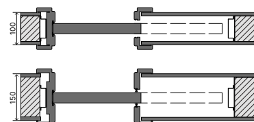
COMPACT 'TUNNEL' FRAMES ARE DEDICATED FOR WALL THICKNESSES 100 MM AND 150 MM
